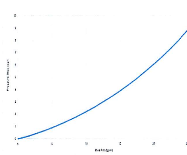
5/8" Headloss Curve
