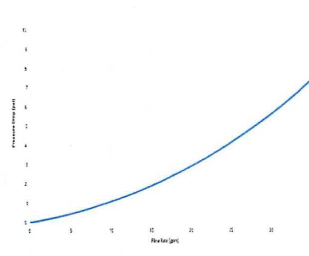
3/4" Headloss Curve
