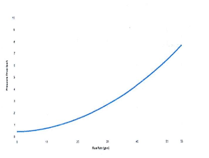
1" Headloss Curve
